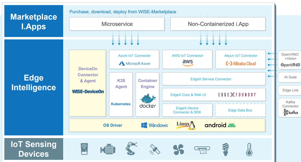
Ei software integration architecture
